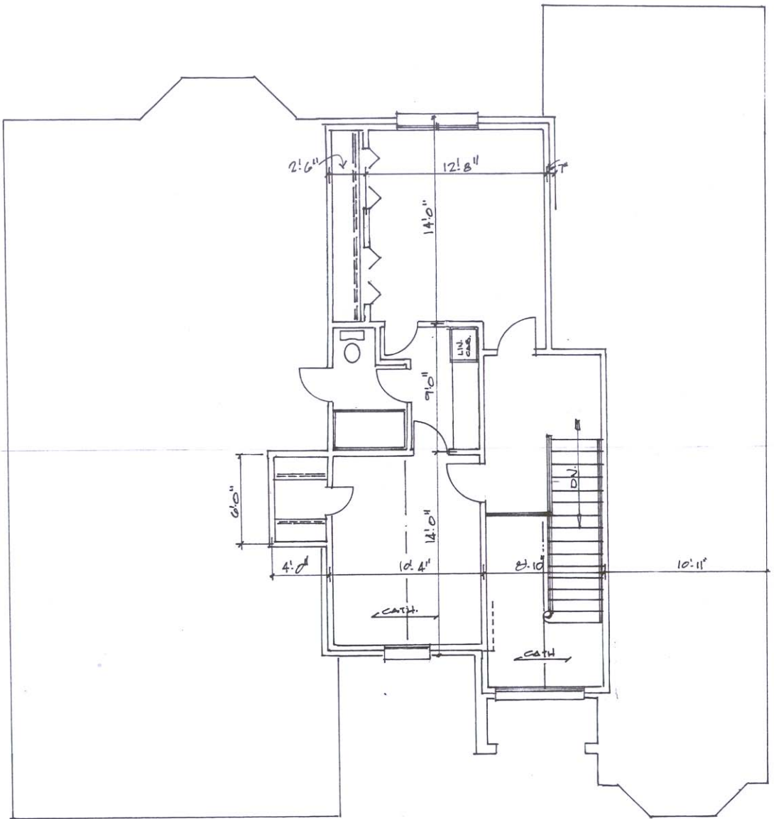
SECOND FLOOR PLAN SCALE: 1/4" = 1'-0"
